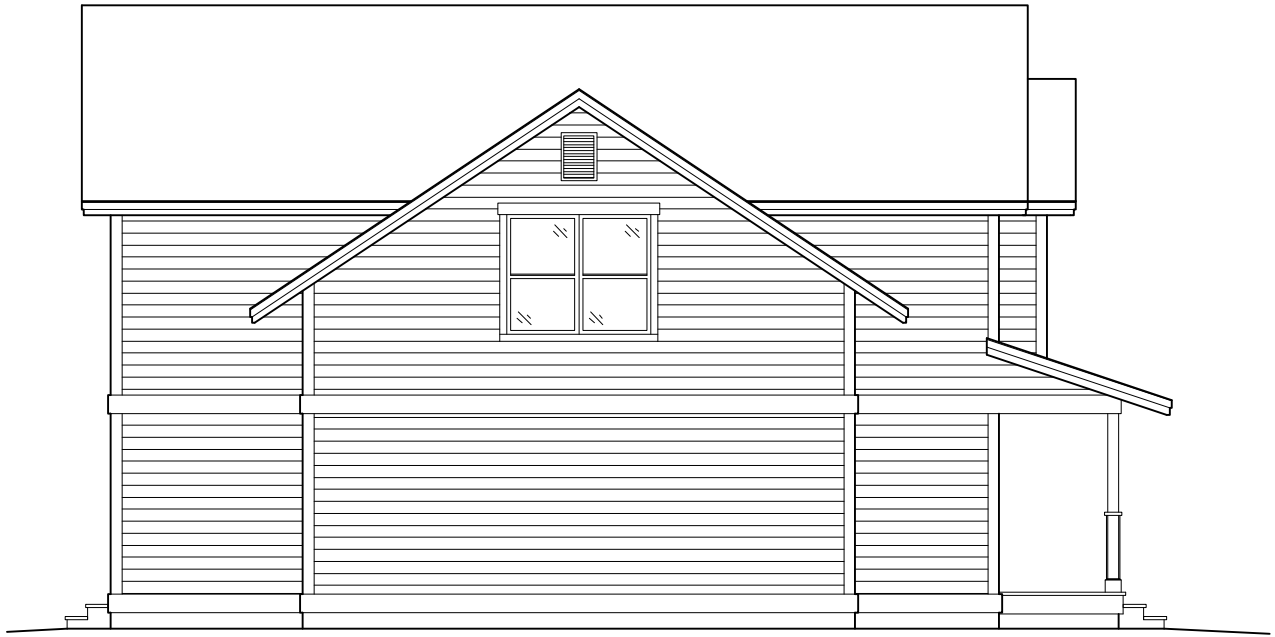
LEFT ELEVATION
